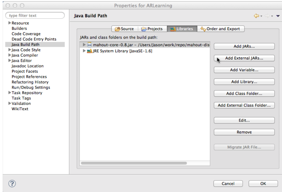
Figure 6-2: Adding the required JAR files
