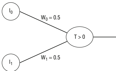
Figure 5-5: AND gate perceptron
