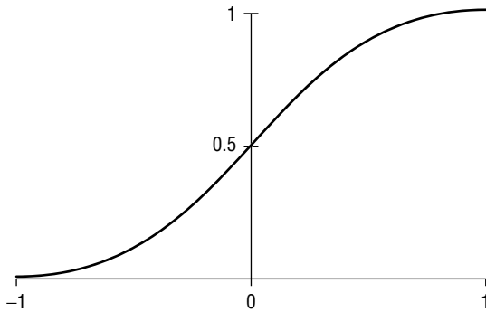
Figure 5-4: Sigmoid function
