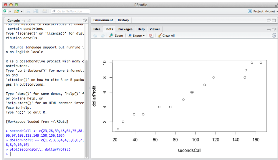
Figure 12-9: Seconds/dollar plot
