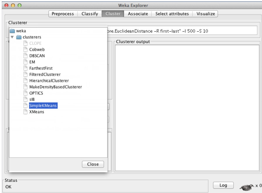
Figure 8-7: Selecting SimpleKMeans
